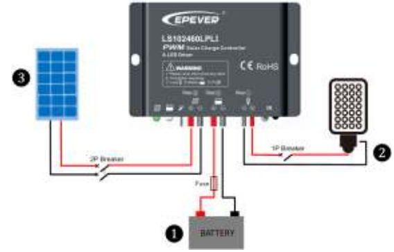
Figure 2 Wiring
